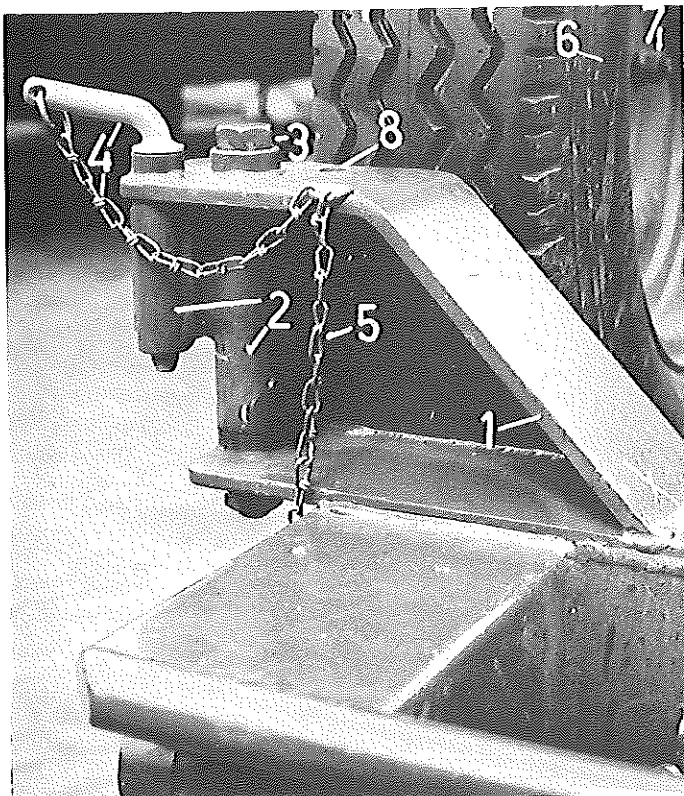
AFB.34 RESERVEWIELDRAGER.
